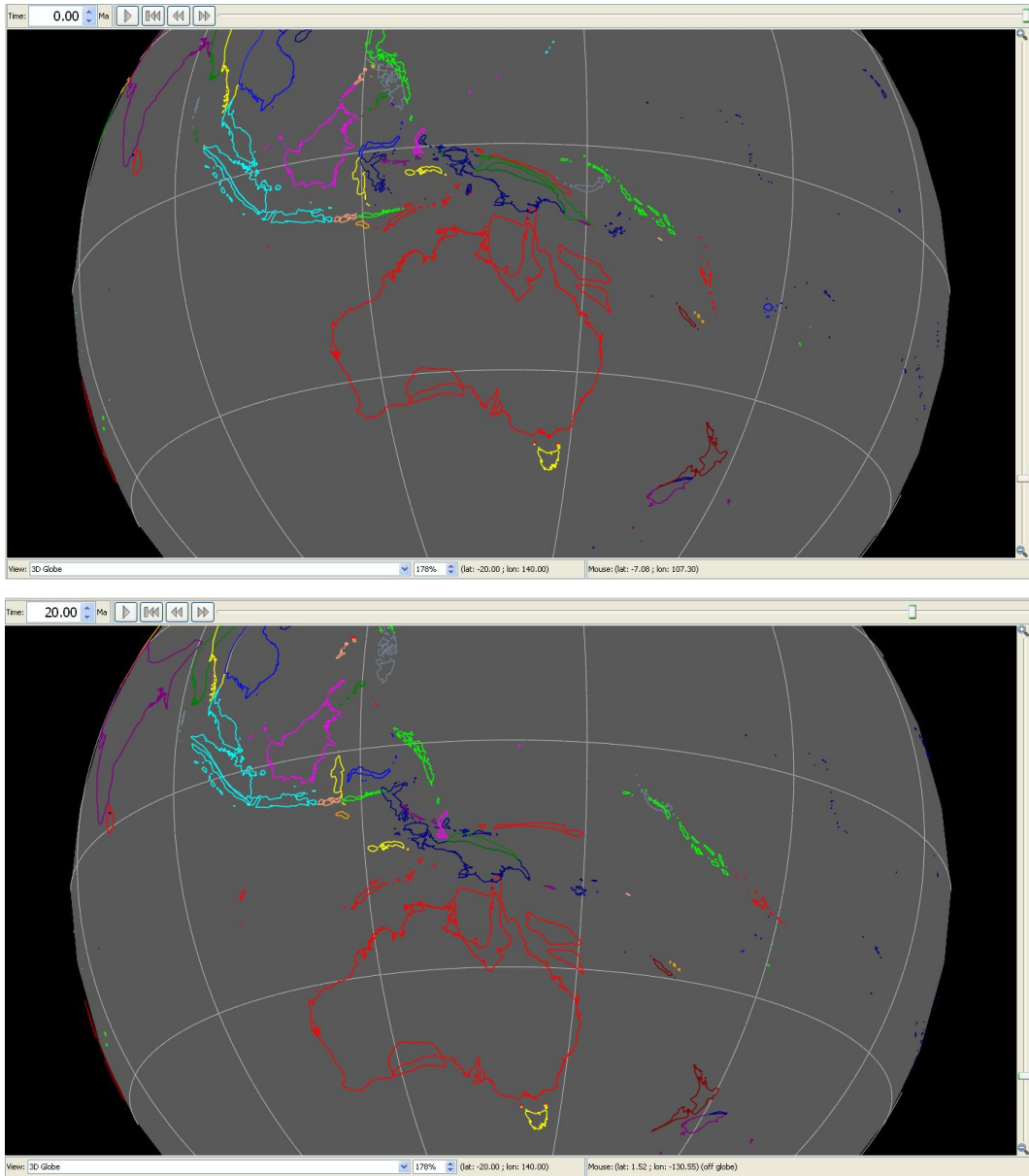
Figure 6. View of the Australian region showing that the basins are moving fixed to Australia.
