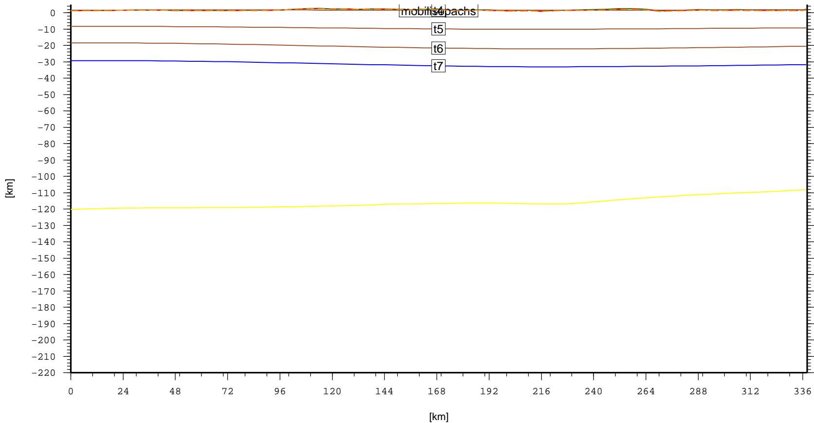
Cross section – AFR.Abbay_BlueNileBasin (topo, laske sedthick, t4, t5, t6, t7)
