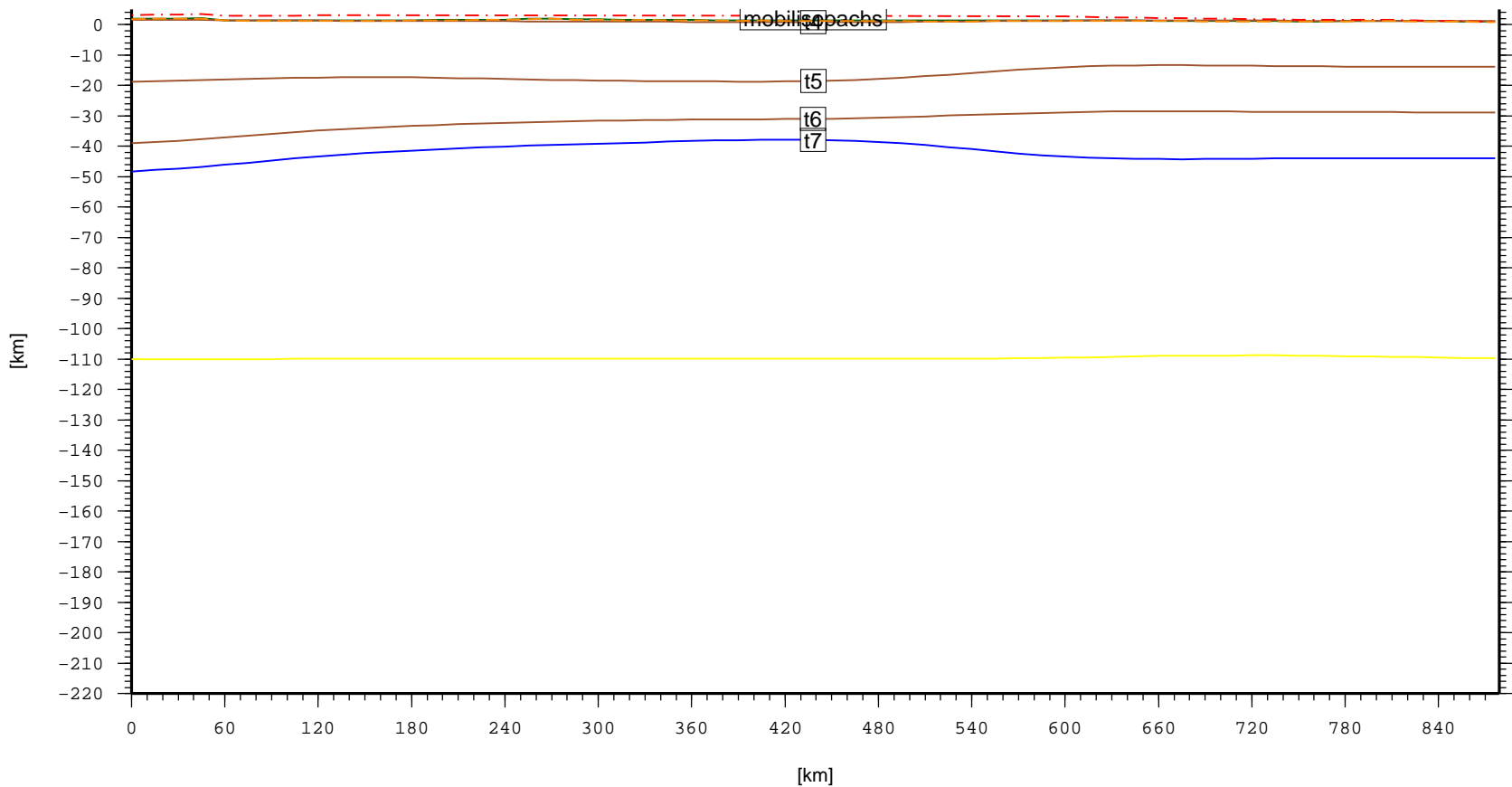
Cross section – CHN.CentralGobiBasin (topo, laske sedthick, t4, t5, t6, t7)
