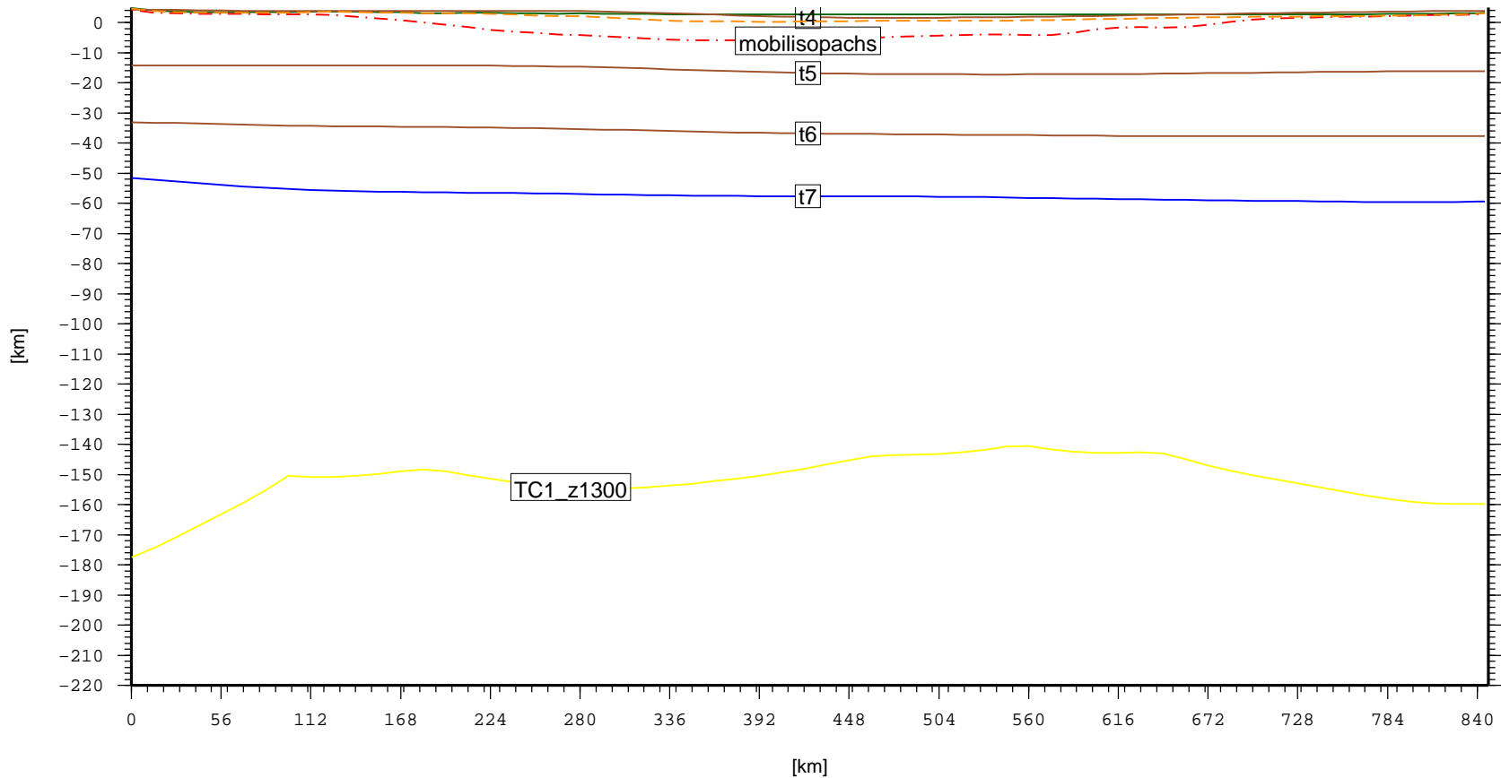
Cross section – CHN.Qaidam_TsaidamBasin (topo, laske sedthick, t4, t5, t6, t7)
