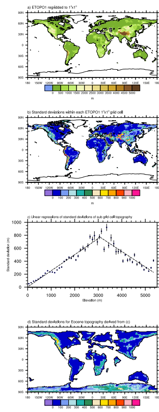
Fig. 2. Estimating the standard deviation of sub grid cell elevations for the Eocene. (a) ETOP01 topography downsampled from its native 1' \times 1' resolution to 1^\circ \times 1^\circ . (b) Standard deviation of 1' \times 1' elevations inside each 1^\circ \times 1^\circ grid cell. (c) Standard deviations from (b) area-weight averaged into 100 m bins and plotted against corresponding elevation. Standard error for each bin is plotted. Dotted lines represent linear regressions between sea-level and 3000 m, and 3000 m and 5500 m. (d) Linear regressions from (c) applied to Eocene topography (Fig. 1c). See text for details.
