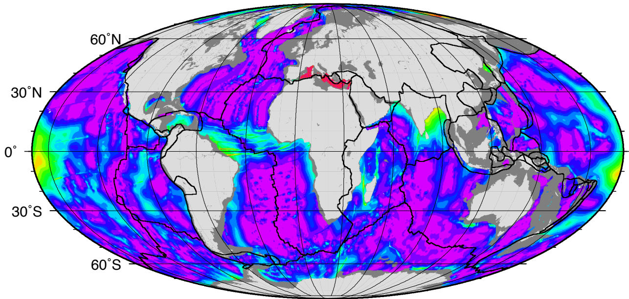
Age of Oceanic Lithosphere [m.y.]
